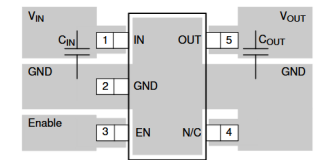
Figure 7-7. DBV Package (SOT-23) Typical Layout
